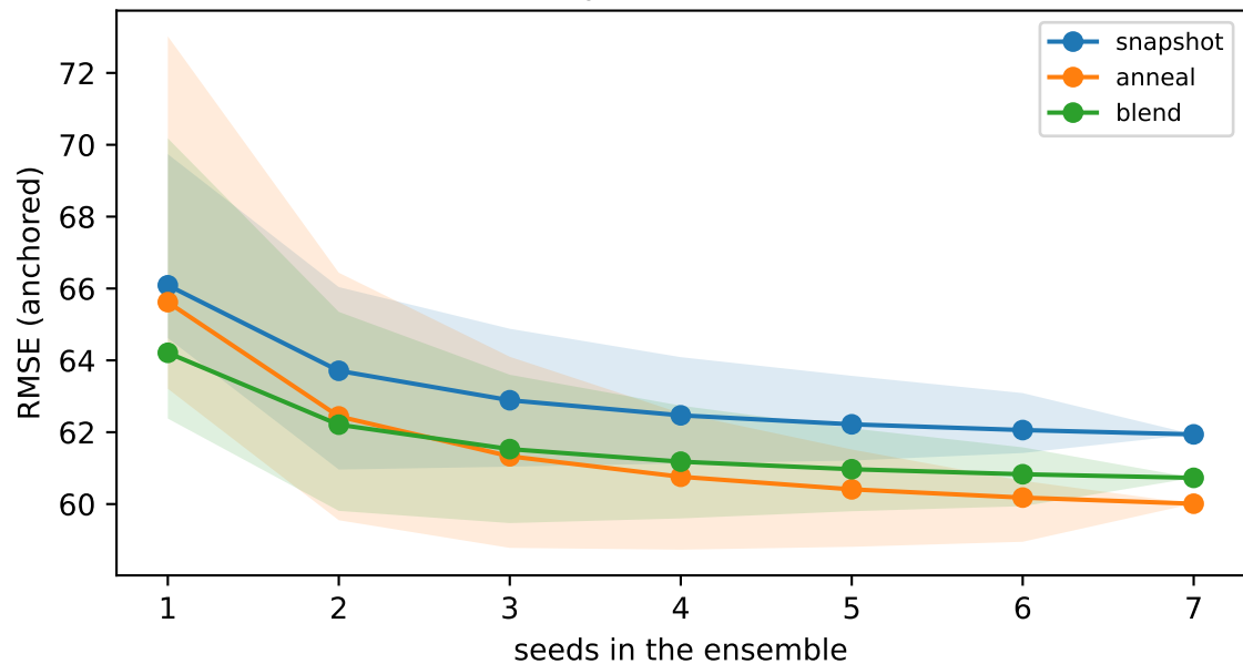
replication fold
