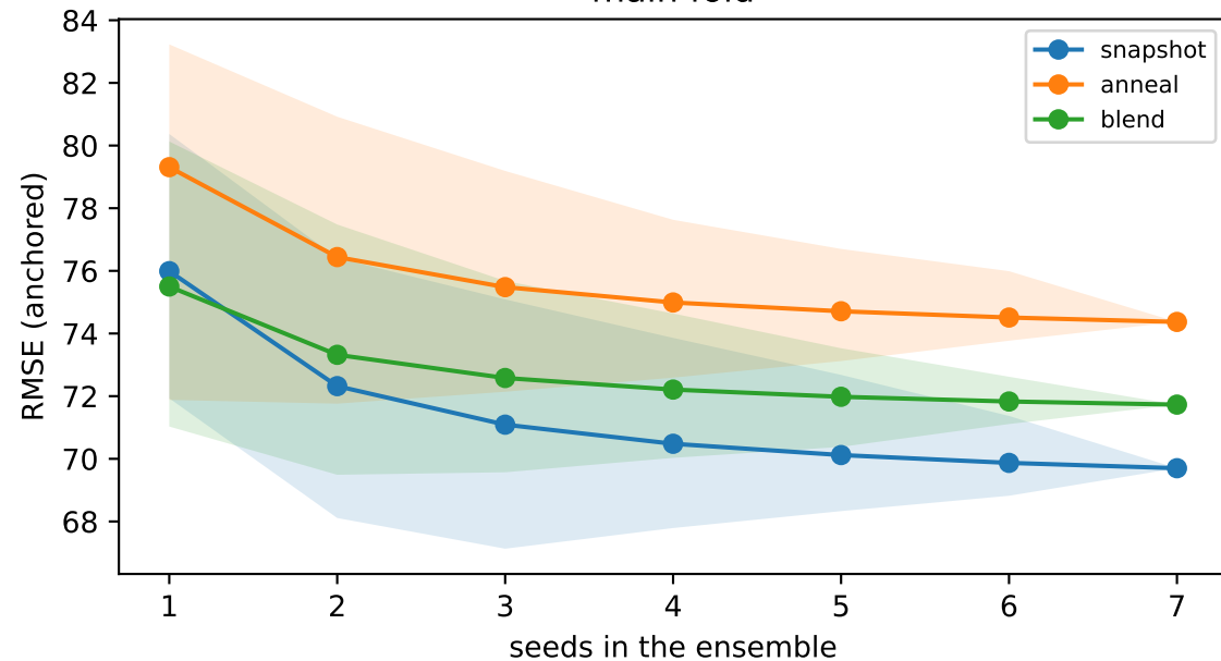
main fold
